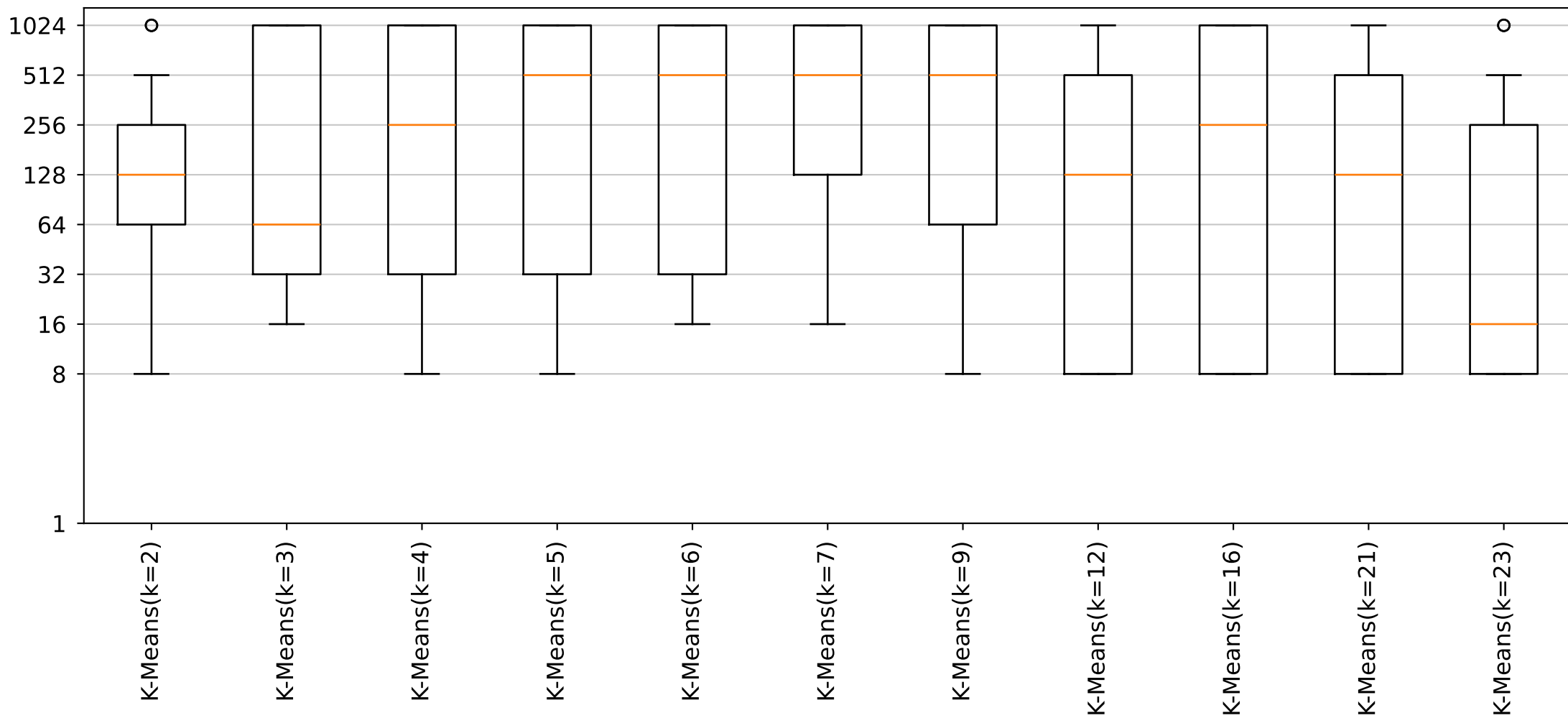
YARA Rules Gram Size Distribution (Cluster6_Size23 dataset)
